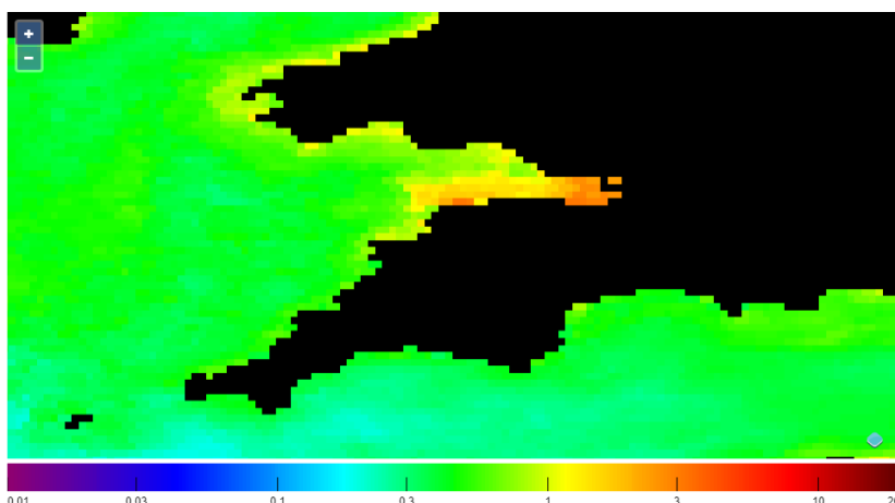
Figure 16 Chlorophyll-a concentration in seawater ( \text{mg m}^{-3} ) August 2018, Bristol Channel and Southern Celtic Sea, Ocean Colour-CCI (Plymouth Marine Laboratory)
